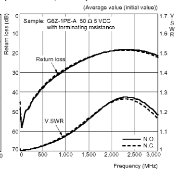
High-frequency Characteristics at 50 Ω (Return Loss, V.SWR)
