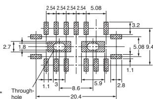
PCB Mounting Holes (Top View)
