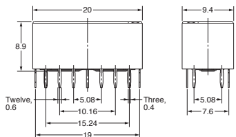
G6WK-1F
