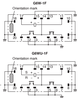
Terminal Arrangement/Internal Connections (Top View)
