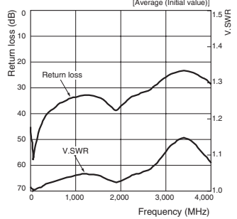
High-frequency Characteristics (Return Loss)
