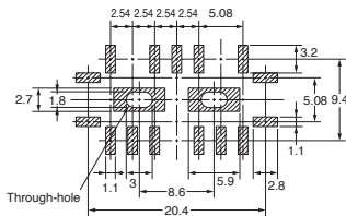
PCB Mounting Holes (Top View) Tolerance: \pm 0.1 mm
