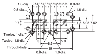
PCB Mounting Holes (Bottom View)
